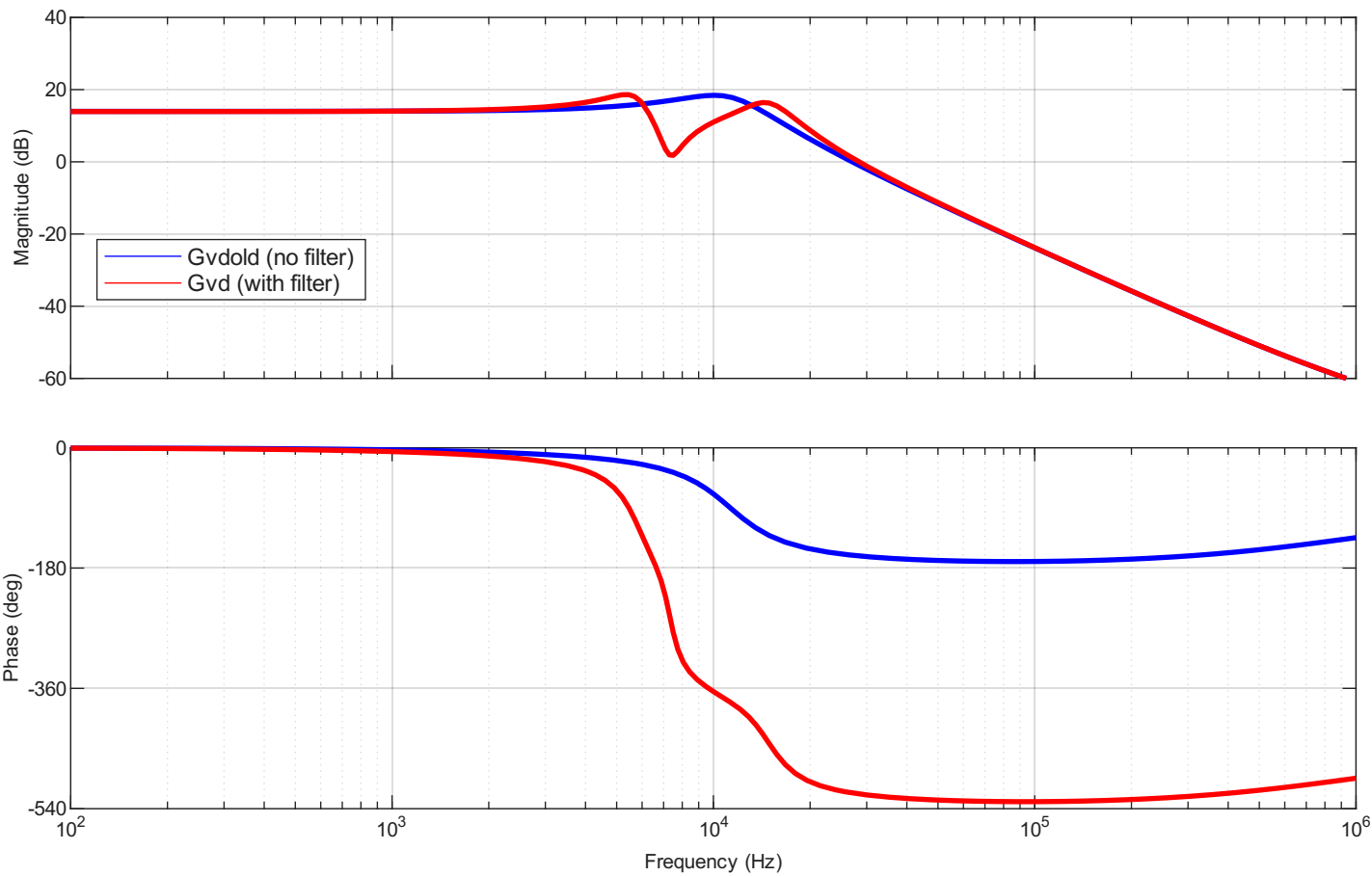
Gvdold no filter (blue) vs Gvd with filter (red)
